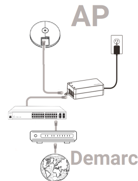
Figure2: AP to CB Topology
