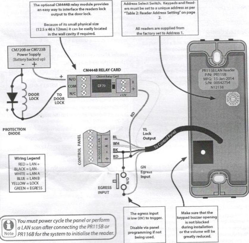
Figure 4: Connection Diagram
